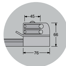
MOD. 4274G End fitting, 2 sheaves (D = 45 mm) and becket
