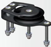
MOD. 00811 FOOT BLOCK WEIGHT** – 0.29 kg • SWL – 2200 kg SCREWS – 4xØ8 mm (included)
