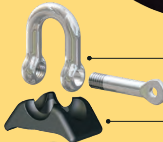
MOD. 008HR HR SHACKLE, Ø8 mm WEIGHT – 62 g SWL – 2200 kg
