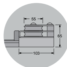
MOD. 4274Z End fitting, 2 sheaves (D = 55 mm) and becket
