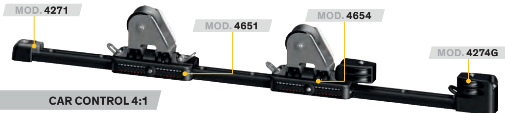
MOD. 4274G End fitting, 2 sheaves (D = 45 mm) and becket
