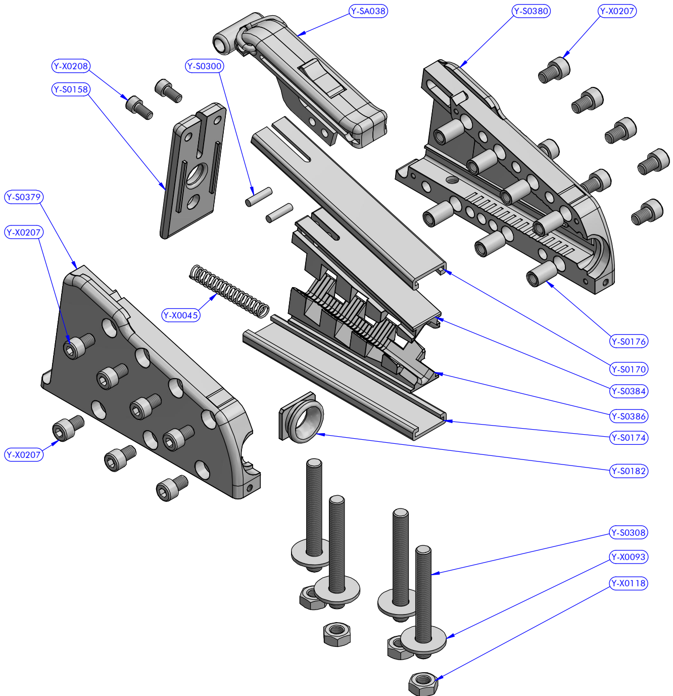
PART LIST - 505.141
